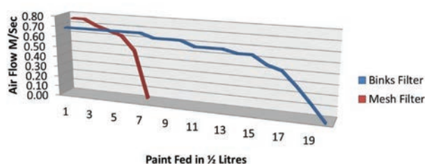
Air Velocity v Paint Loading
